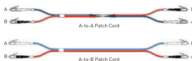
A-to-A and A-to-B Patch Cords
